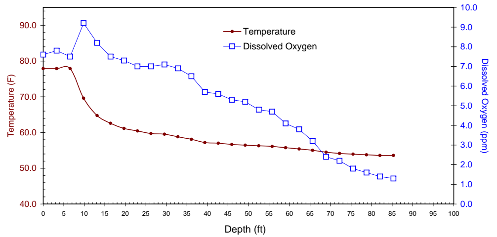
Tellico Reservoir Water Quality at Little TN River Mile 3 - July 8, 2009
